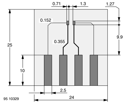
Figure 10. Board for R_{thJA} definition (in mm)
